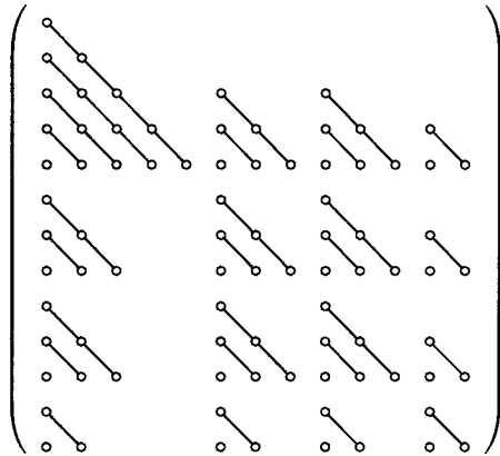
FIG. 1. An element of the centralizer.
