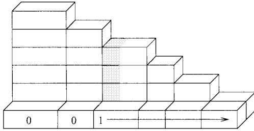
FIG. 5. \mu = (r, 1) .
