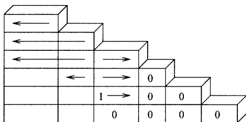
FIG. 4. \mu = (r) .
