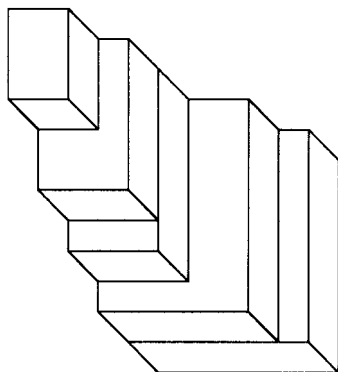
FIG. 2. A three dimensional array.
