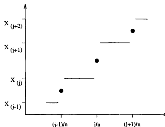
Figure 2. Schematic Representation of \hat{Q}_2(p) .
