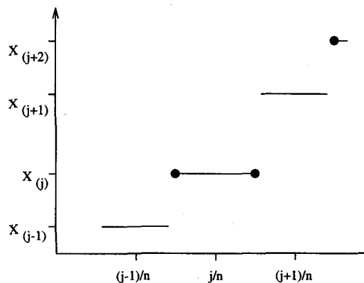
Figure 3. Schematic Representation of \hat{Q}_3(p) ( j Even).
