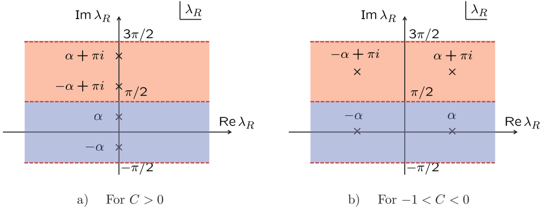
Figure 1: \lambda_R takes values on a cylinder with four punctures.
